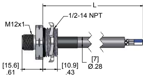
Male Receptacles
