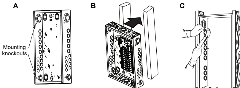
Figure 3: Flush Mounting
