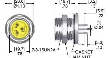
Female Back Mount Receptacle
