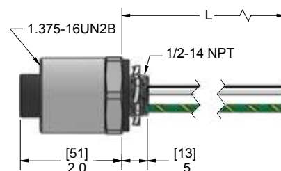
Female Receptacles
