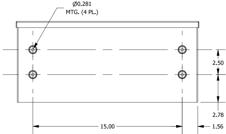
BACK VIEW
