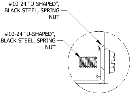
DETAIL A (2 PL.) (LID ATTACHMENT DETAIL)
