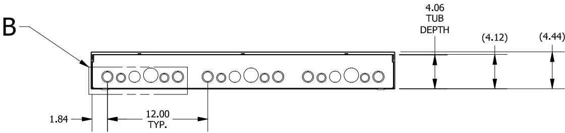
BOTTOM VIEW
