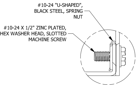
DETAIL A (5 PL.) (LID ATTACHMENT DETAIL)
