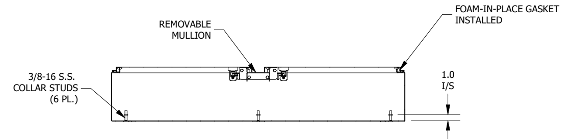
SECTION B-B (INSIDE VIEW OF TOP)
