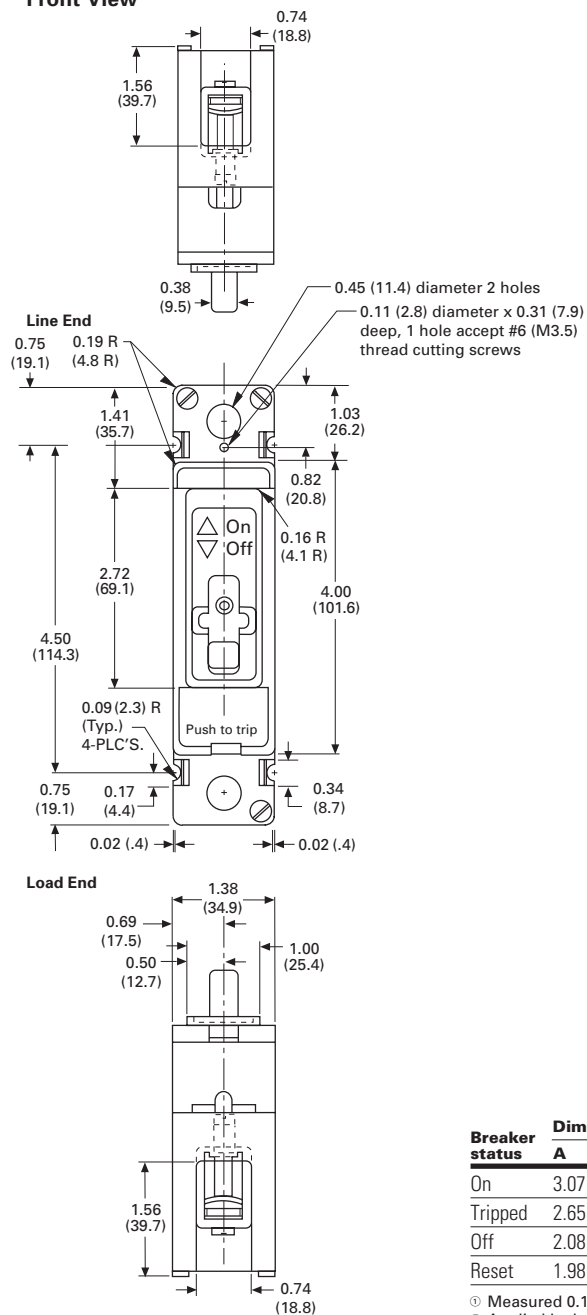
Front View
