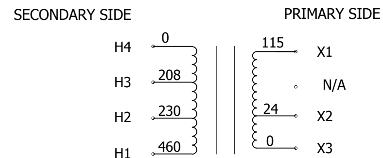
CONNECTION DIAGRAM
