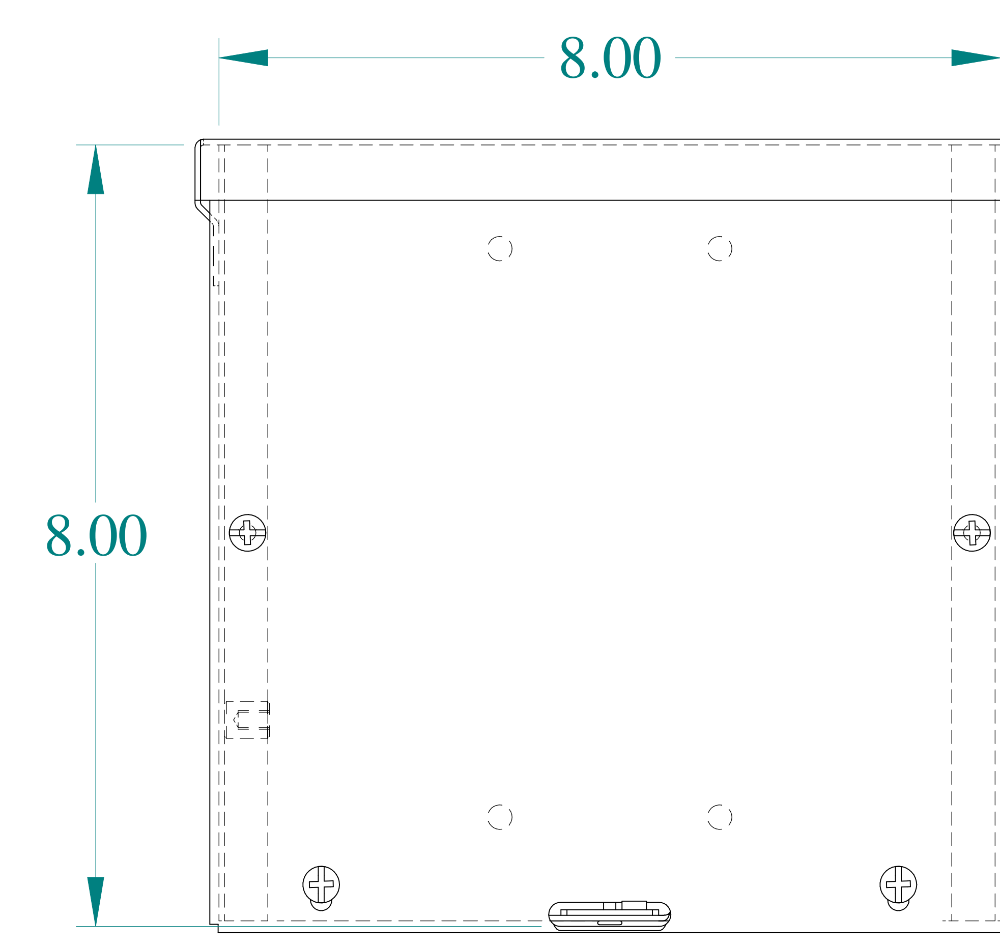
FRONT VIEW
