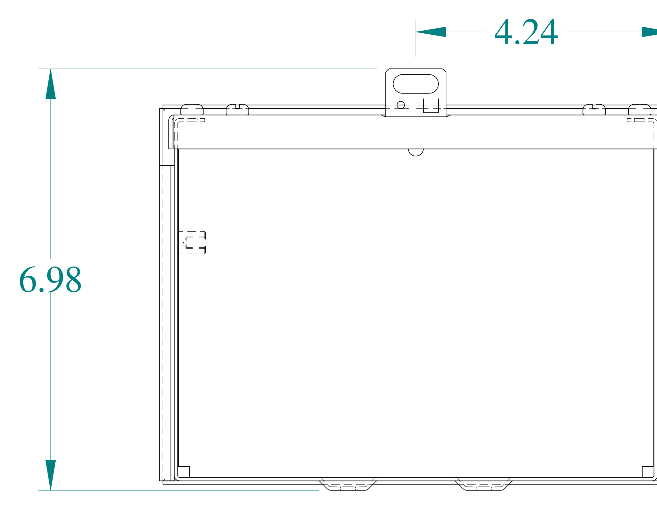
BOTTOM VIEW
