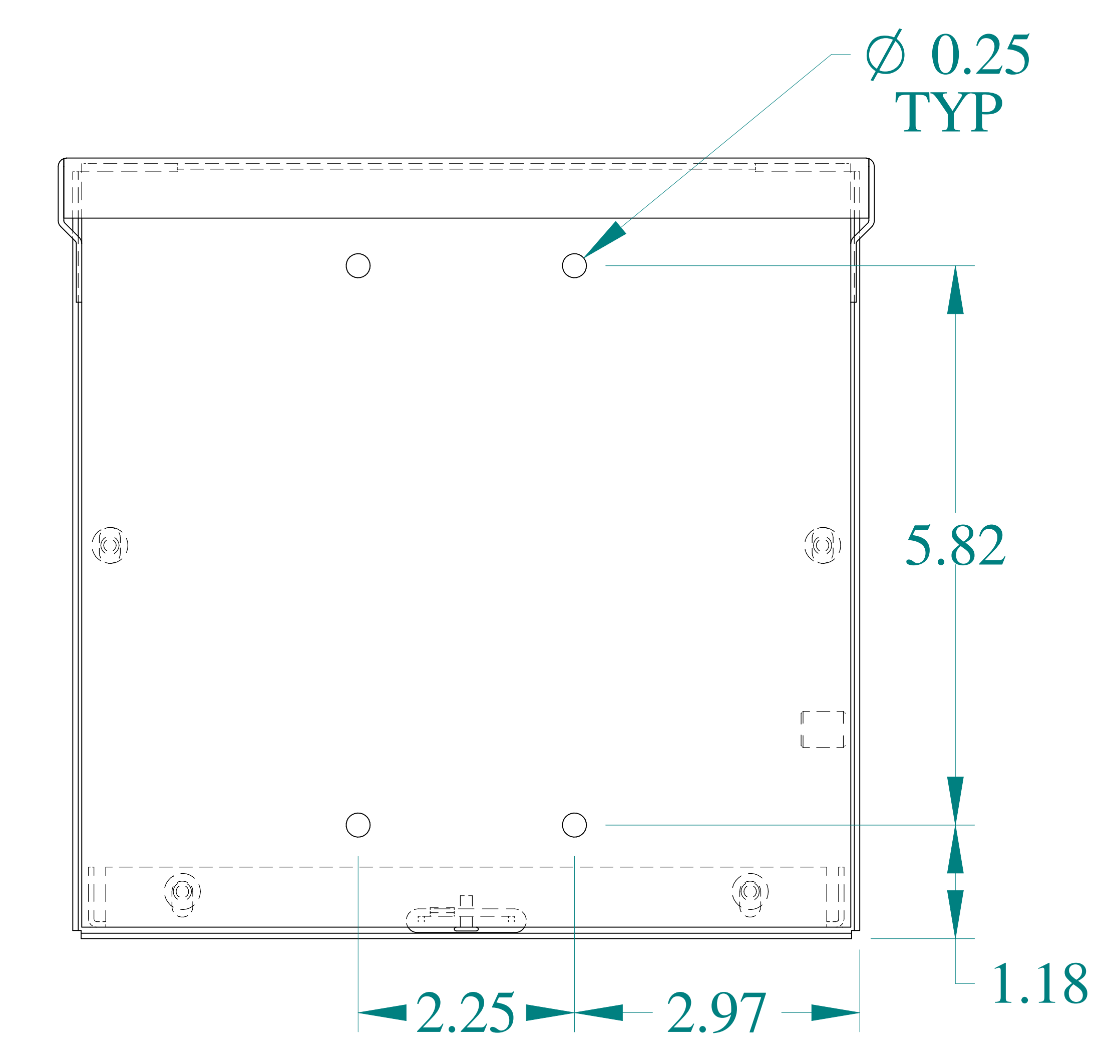
BACK VIEW
