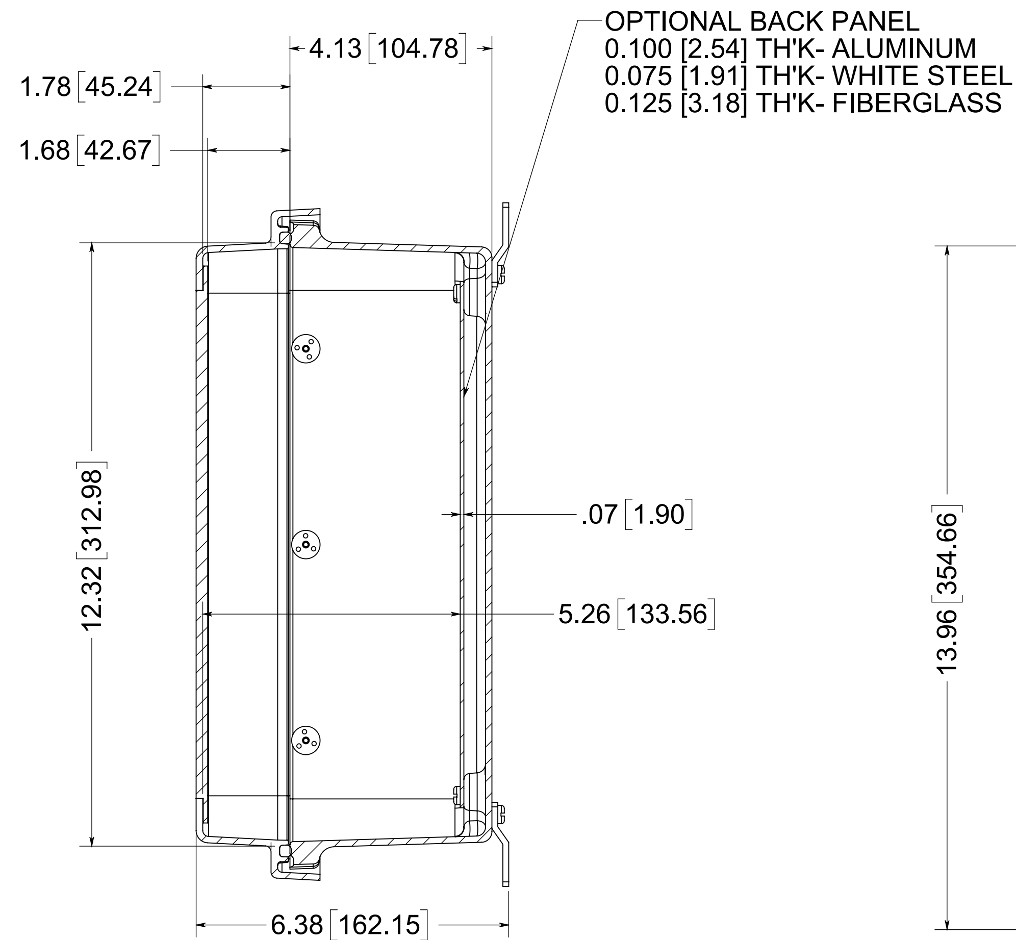
SECTION B-B
