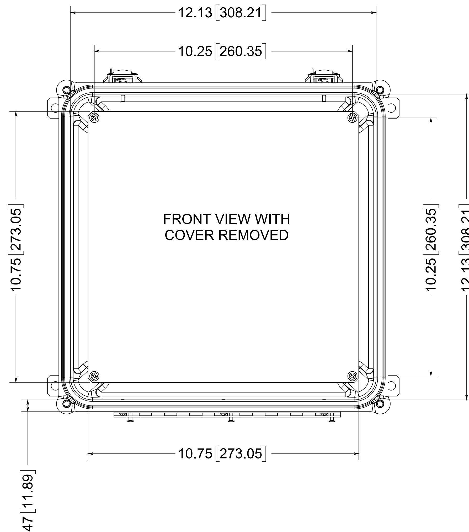
(4X) 316 STAINLESS STEEL FEET
