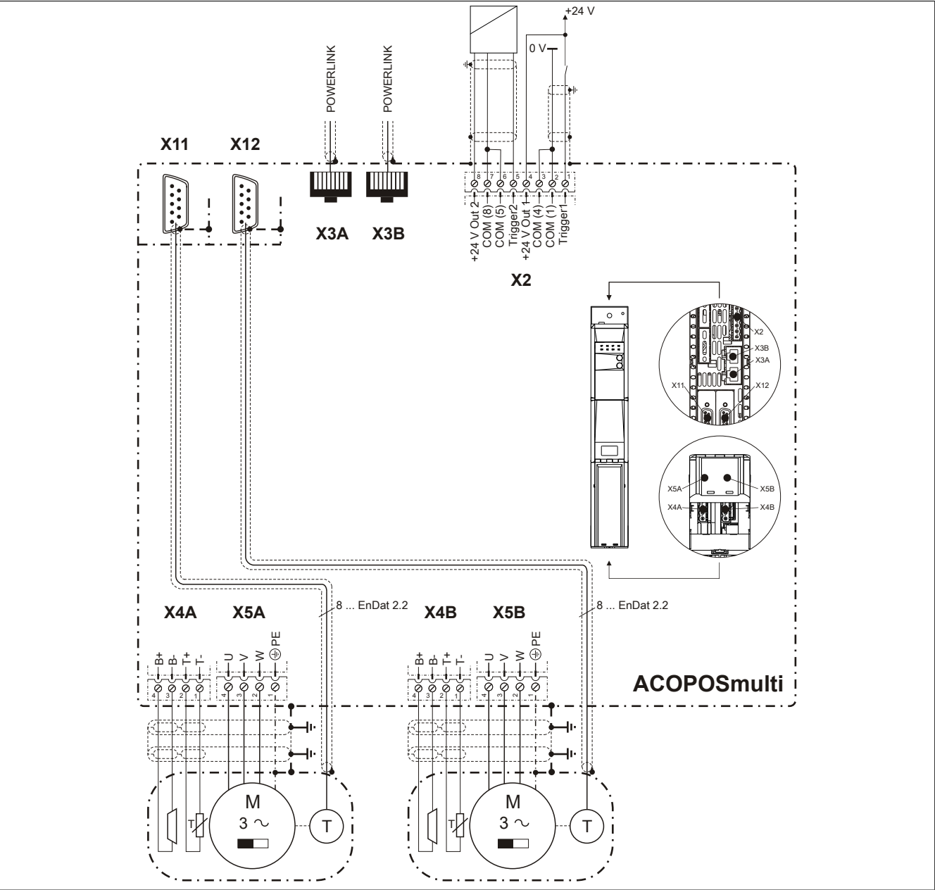
Figure 5: Pinout overview
