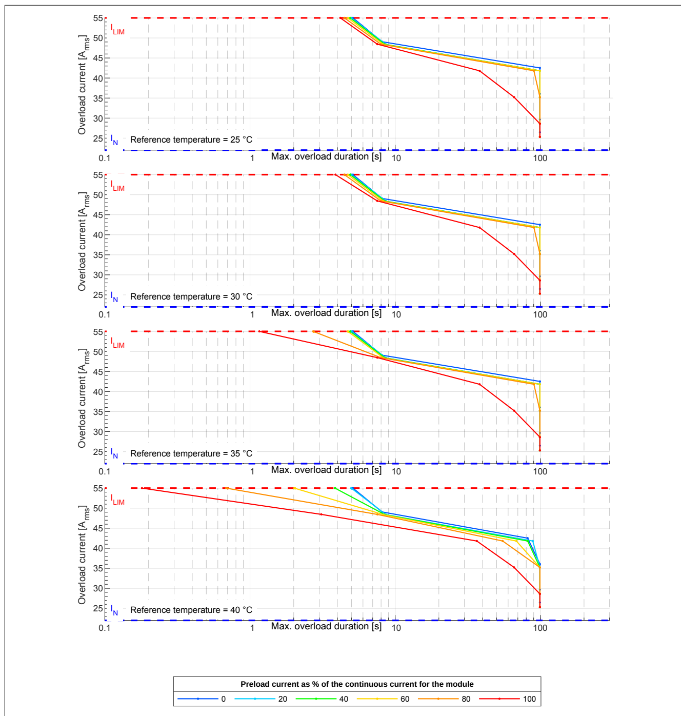
Figure 2: 8BVI0220HWDx.000-1 - Overload characteristics, overload response - ERROR+STOP
