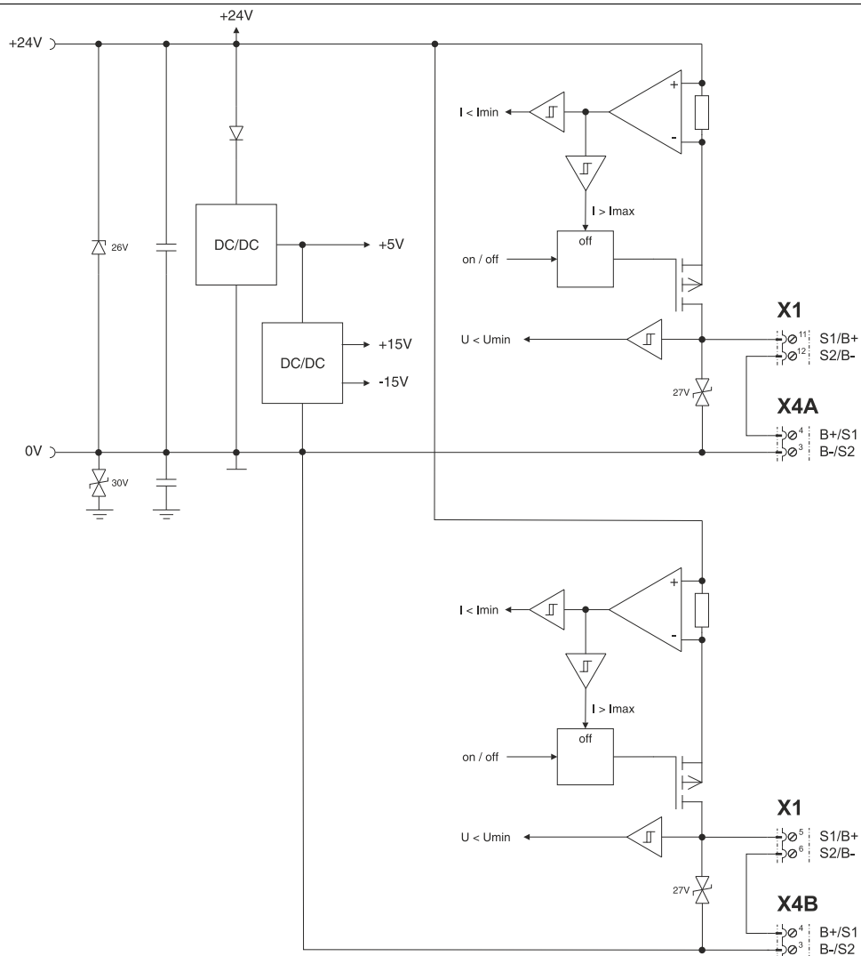
Figure 9: Holding brake
