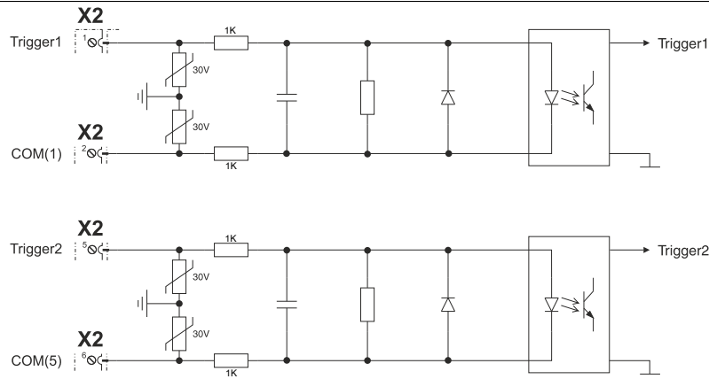
Figure 7: Trigger inputs
