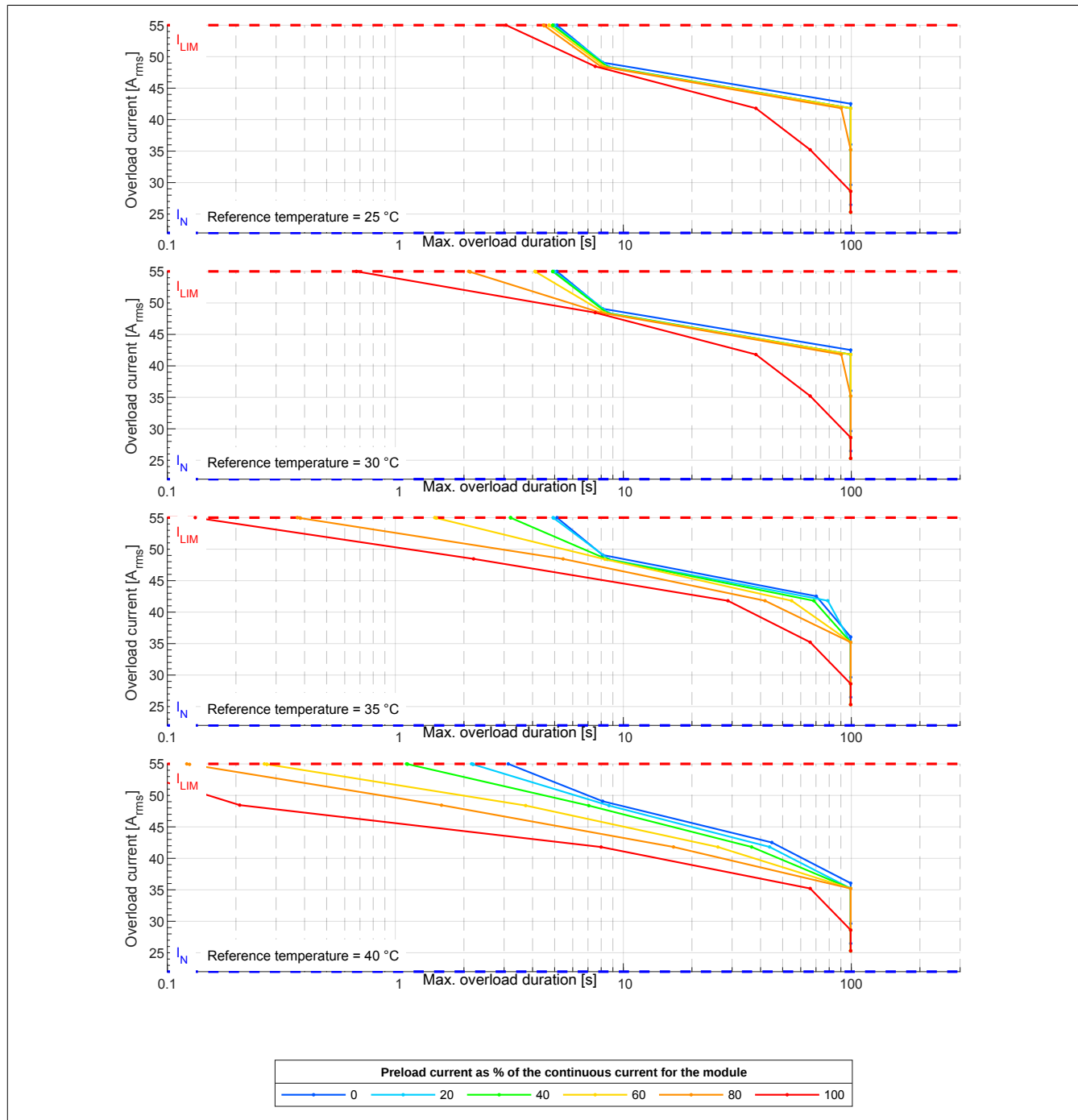
Figure 1: 8BVI0220HWDx.000-1 - Overload characteristics, overload response - WARNING
