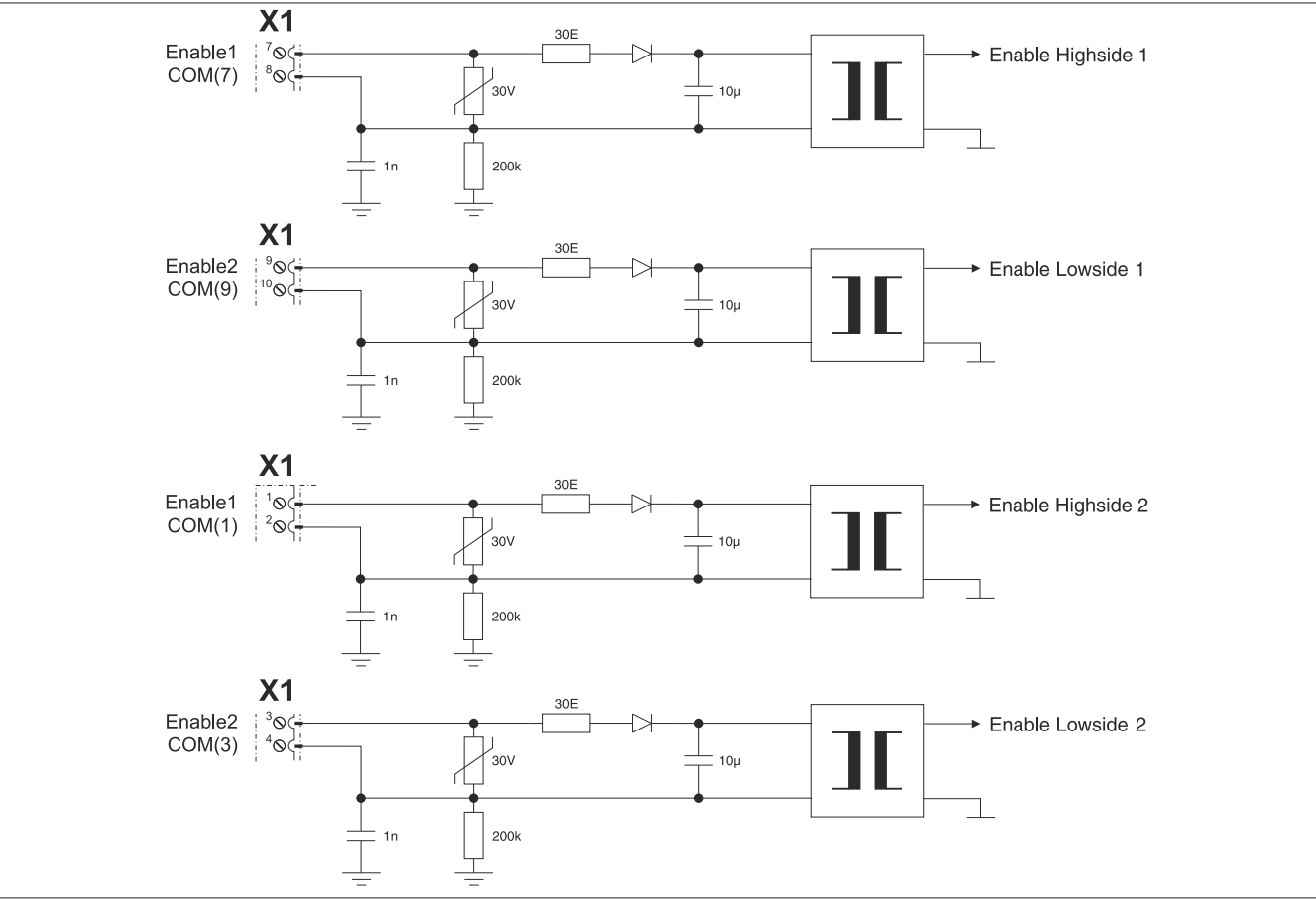
Figure 6: Enable
