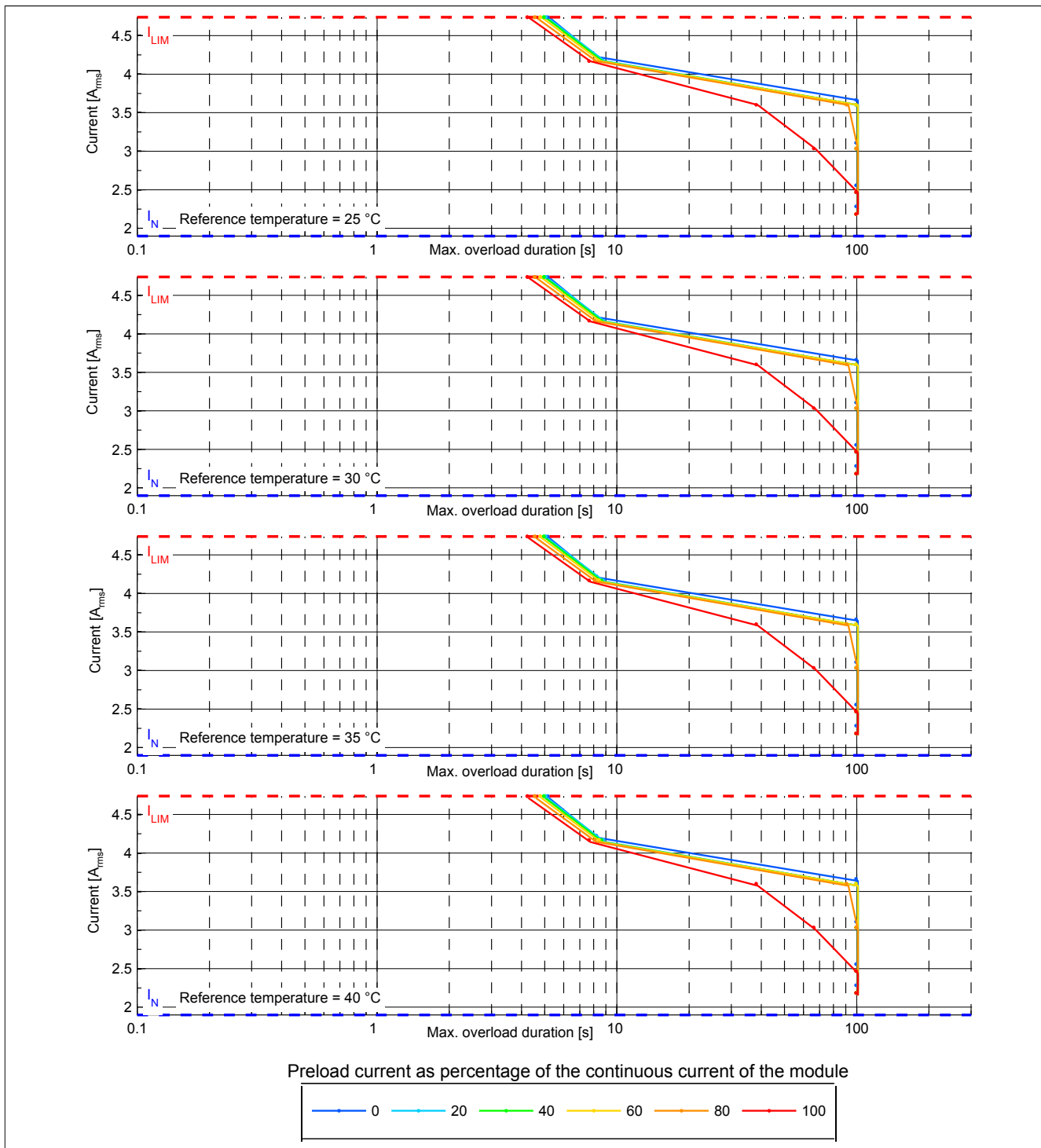
Figure 1: 8BVI0014HWDx.000-1 - Overload characteristics, overload response - WARNING
