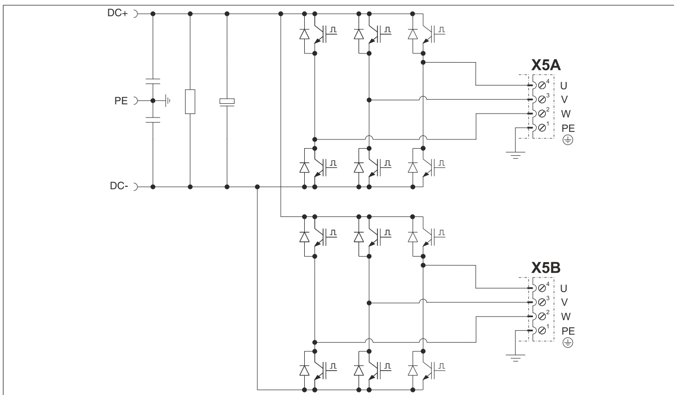
Figure 9: Motor
