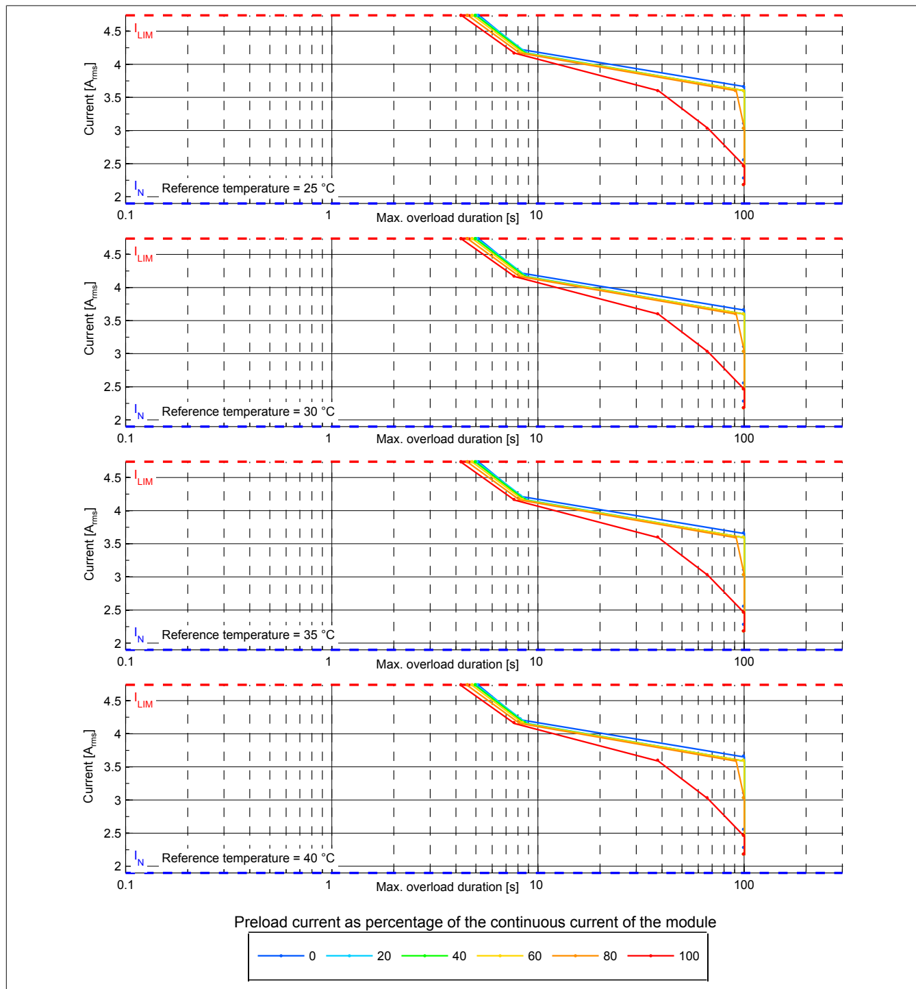
Figure 2: 8BVI0014HWDx.000-1 - Overload characteristics, overload response - ERROR+STOP
