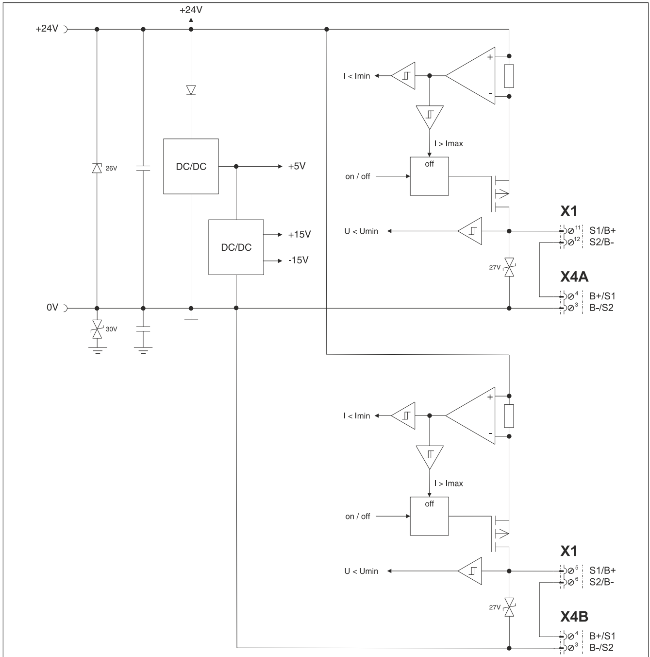
Figure 7: Holding brake
