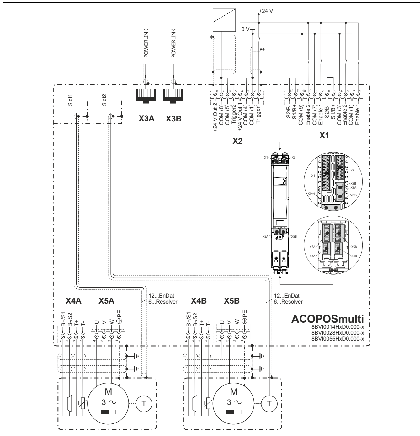
Figure 5: 8BVI0014HxD0.000-x, 8BVI0028HxD0.000-x, 8BVI0055HxD0.000-x - Pinout overview
