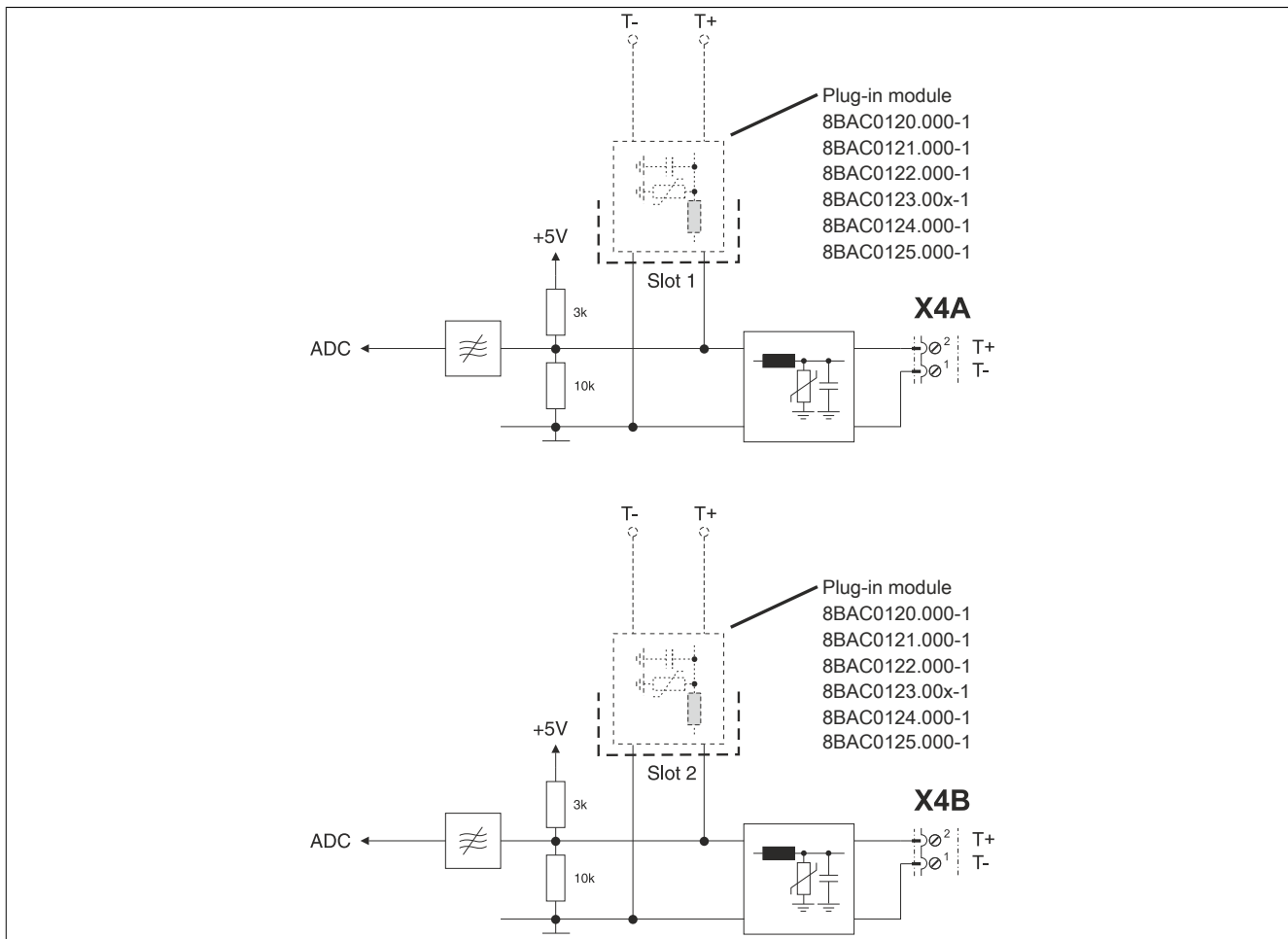
Figure 8: Temperature sensor
