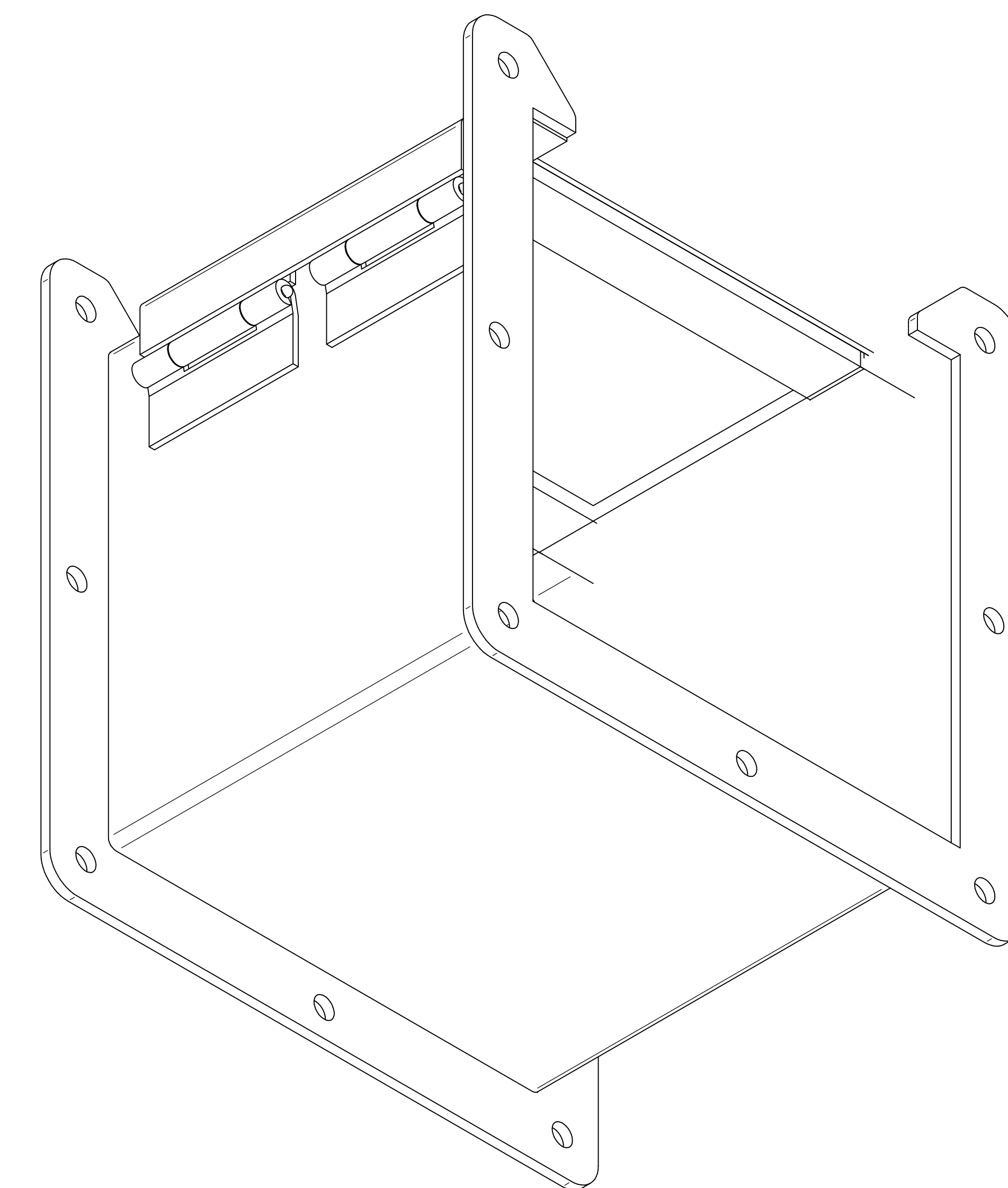
ISOMETRIC VIEWS
