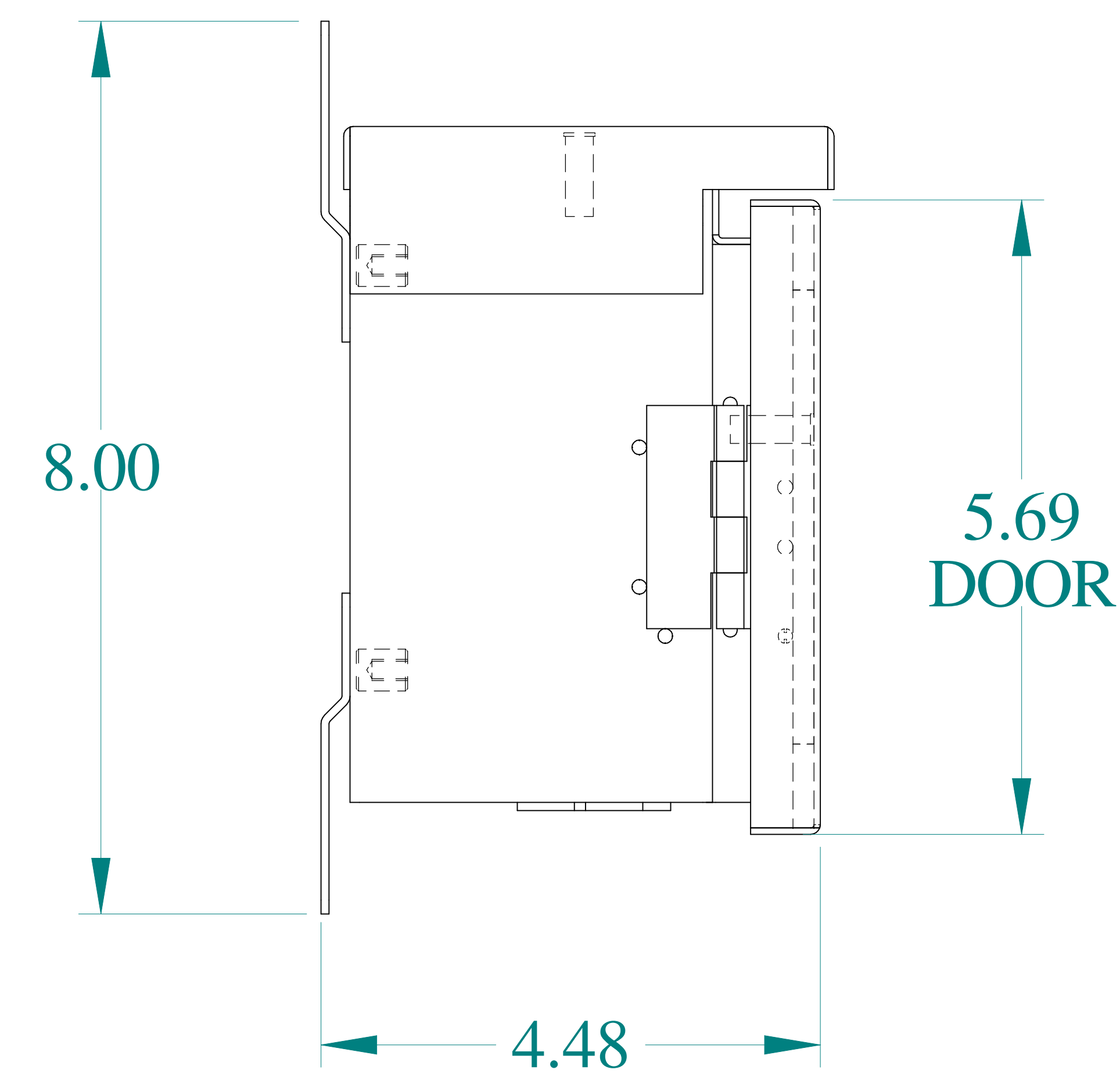
SIDE VIEW
