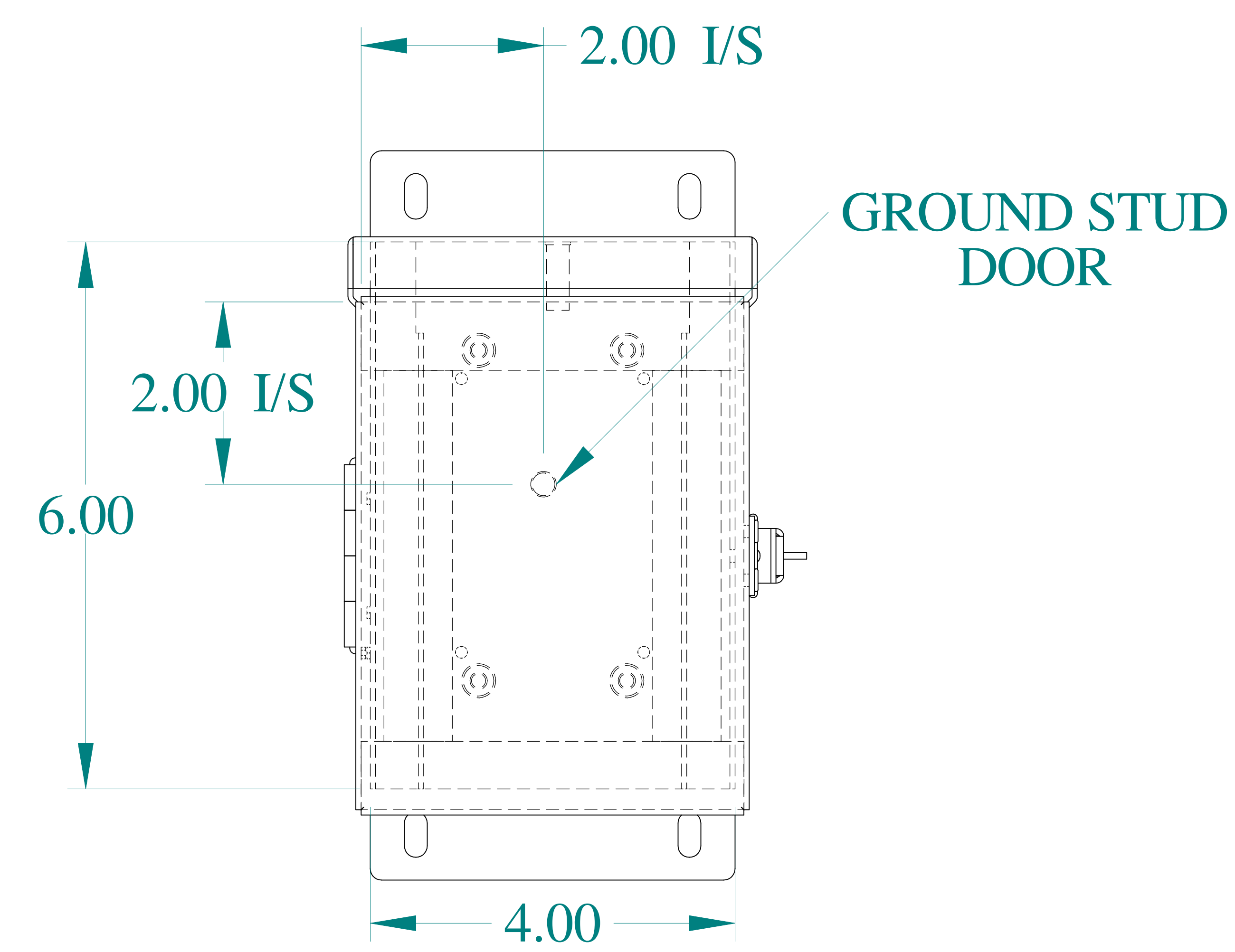
FRONT VIEW
