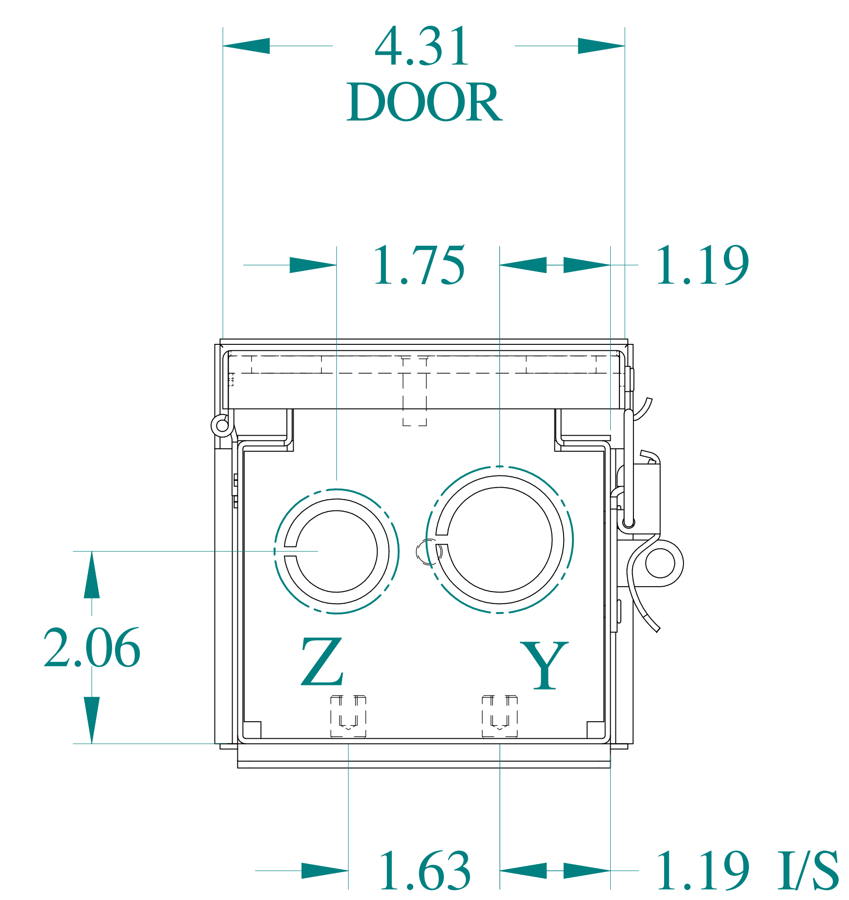
BOTTOM VIEW
