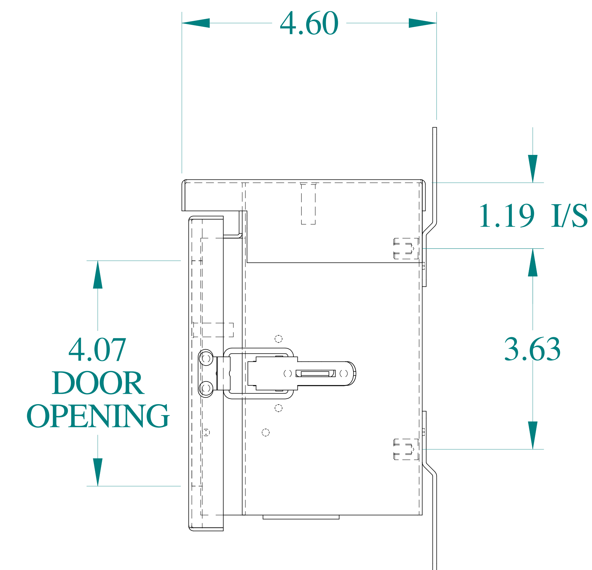
SIDE VIEW
