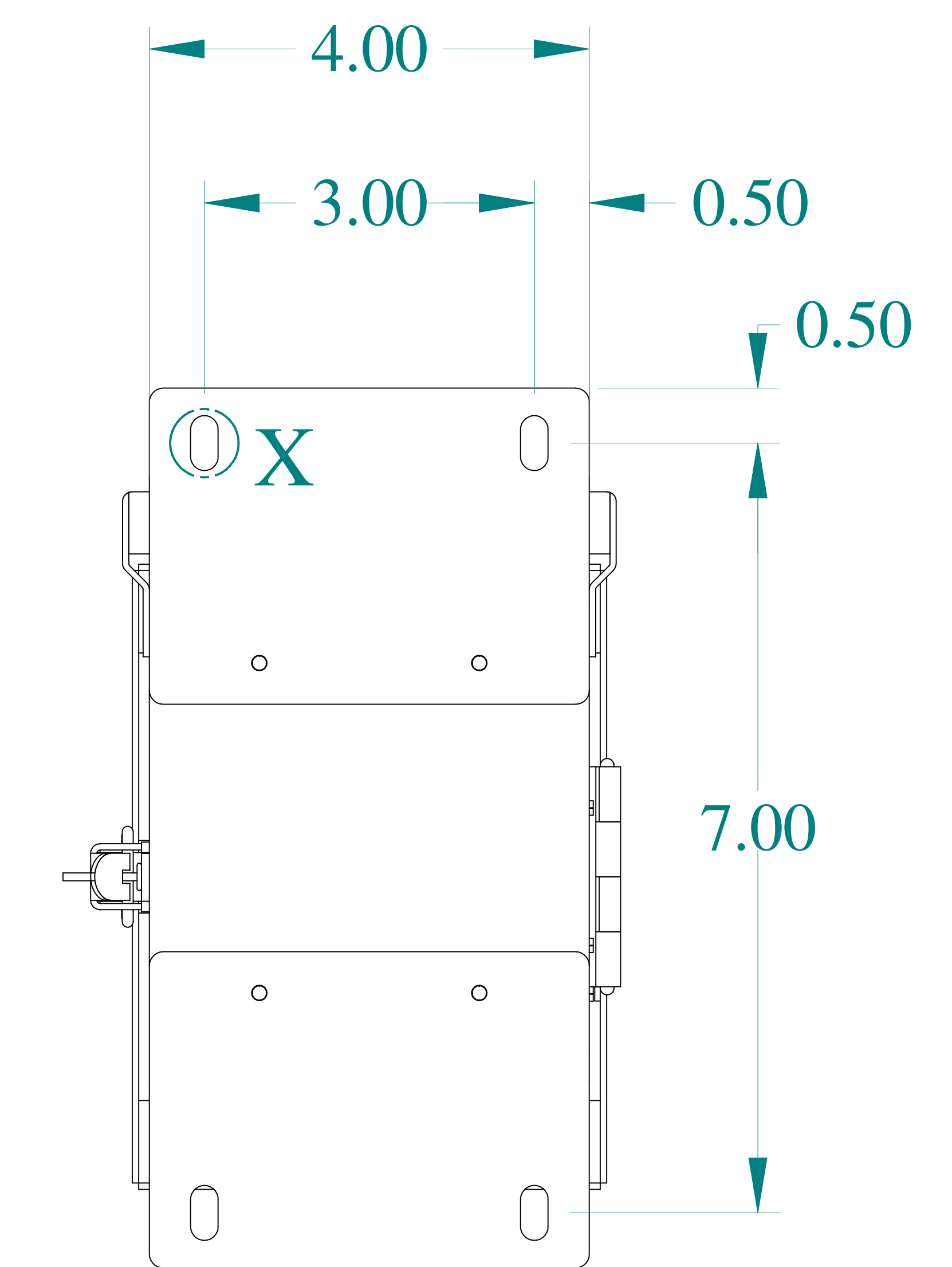
BACK VIEW
