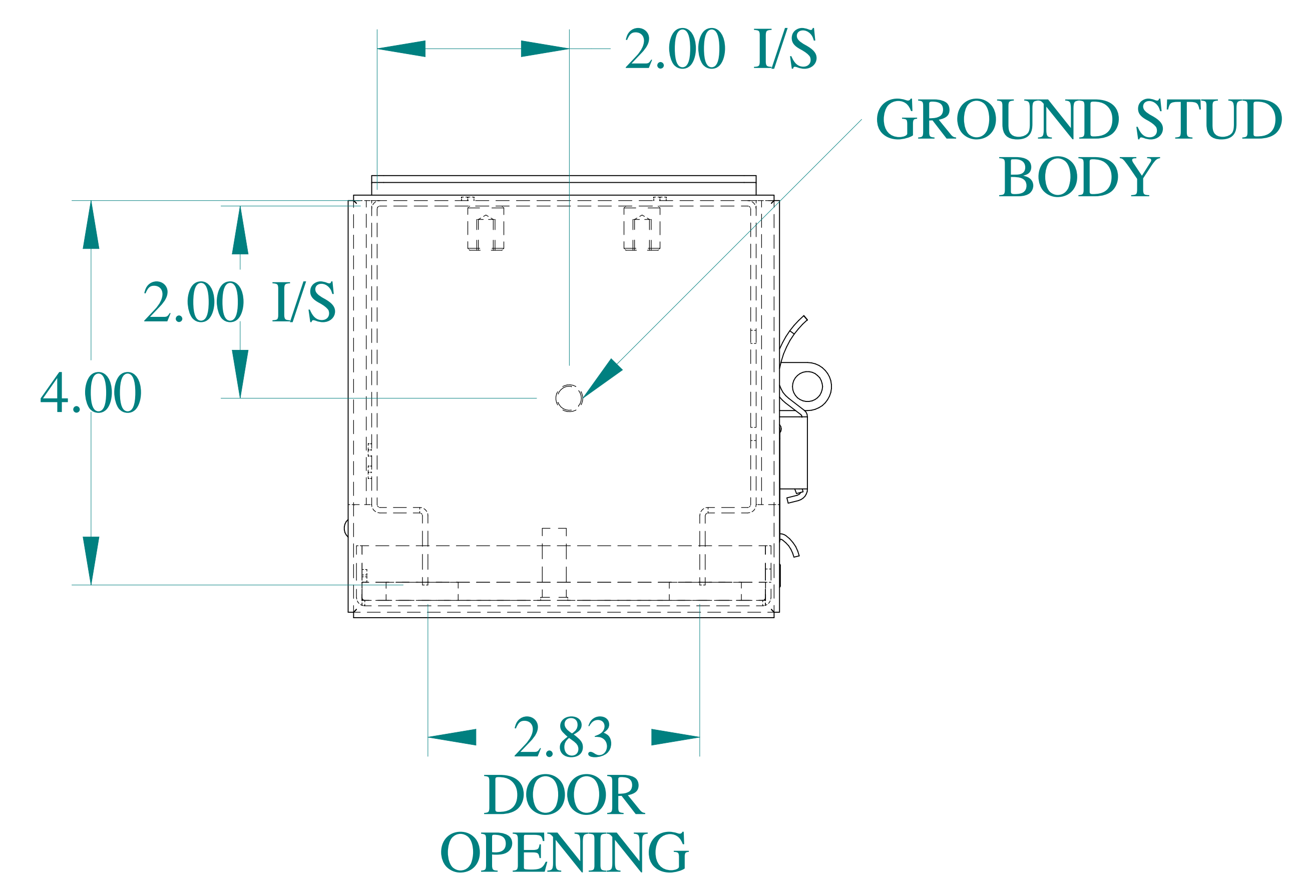
TOP VIEW
