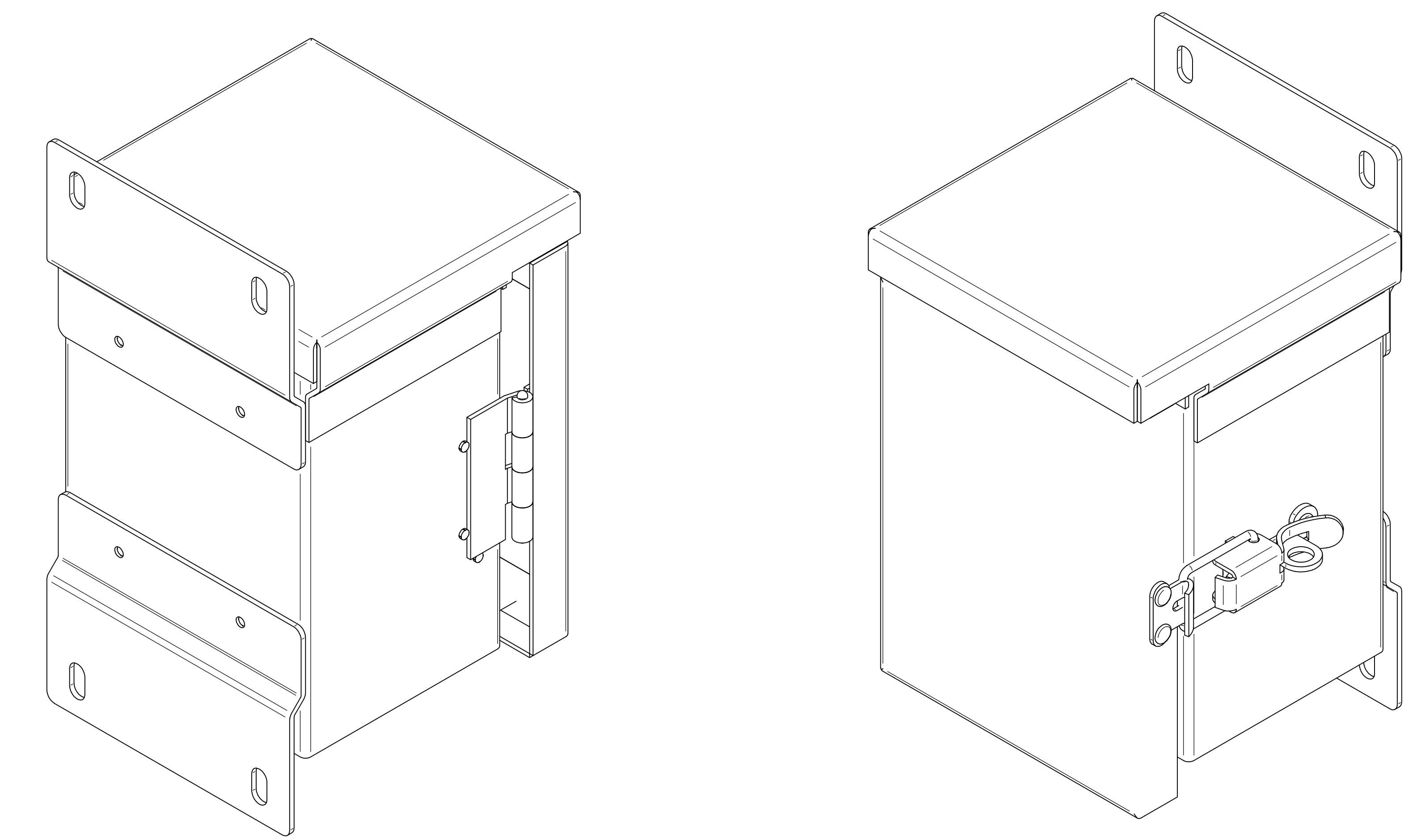
ISOMETRIC VIEWS
