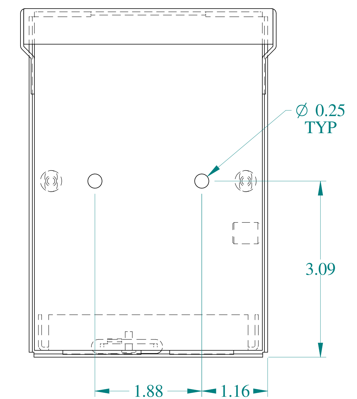
BACK VIEW
