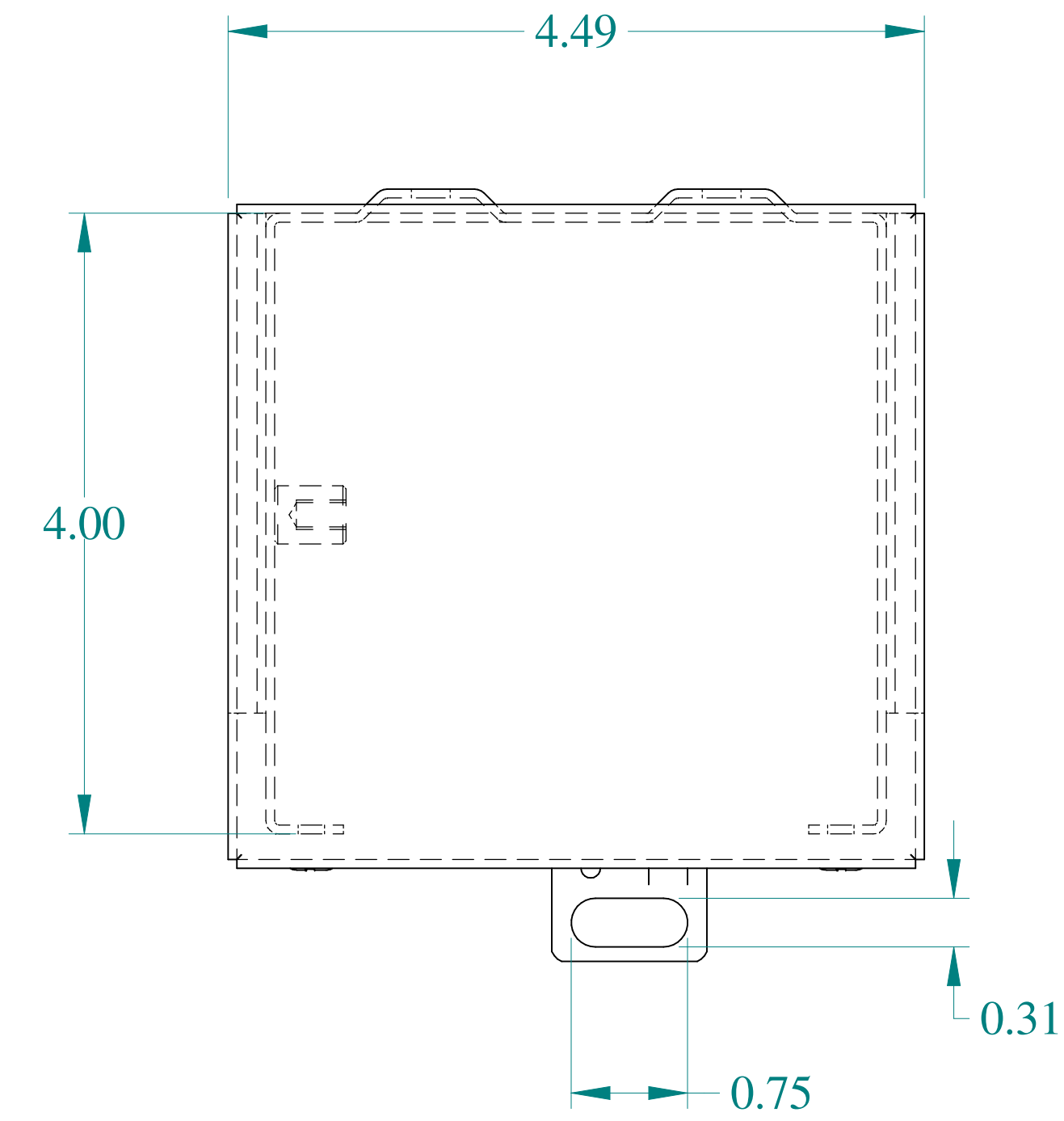
TOP VIEW
