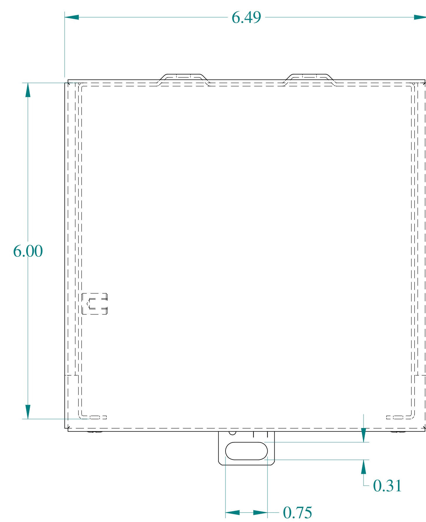
TOP VIEW
