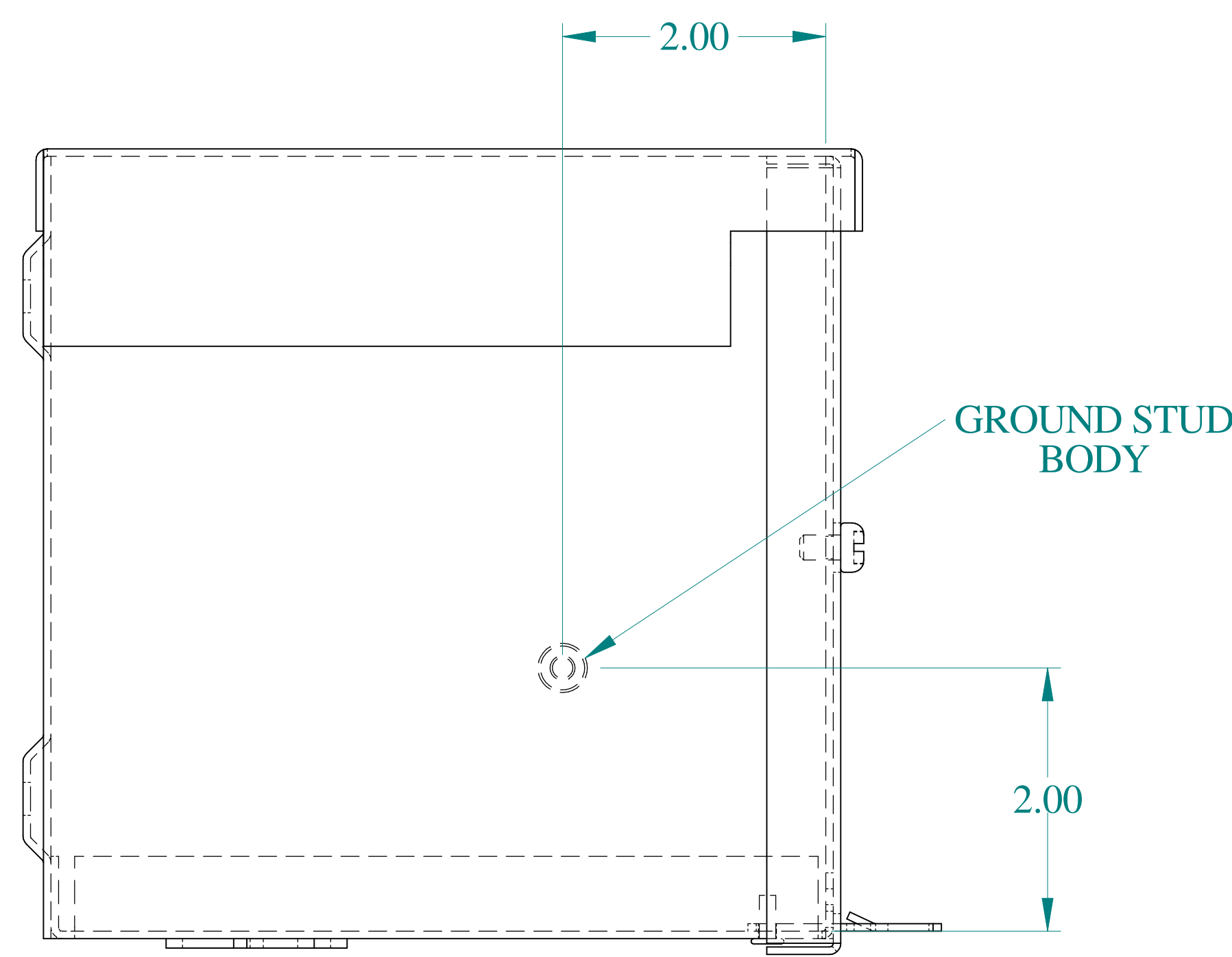
SIDE VIEW
