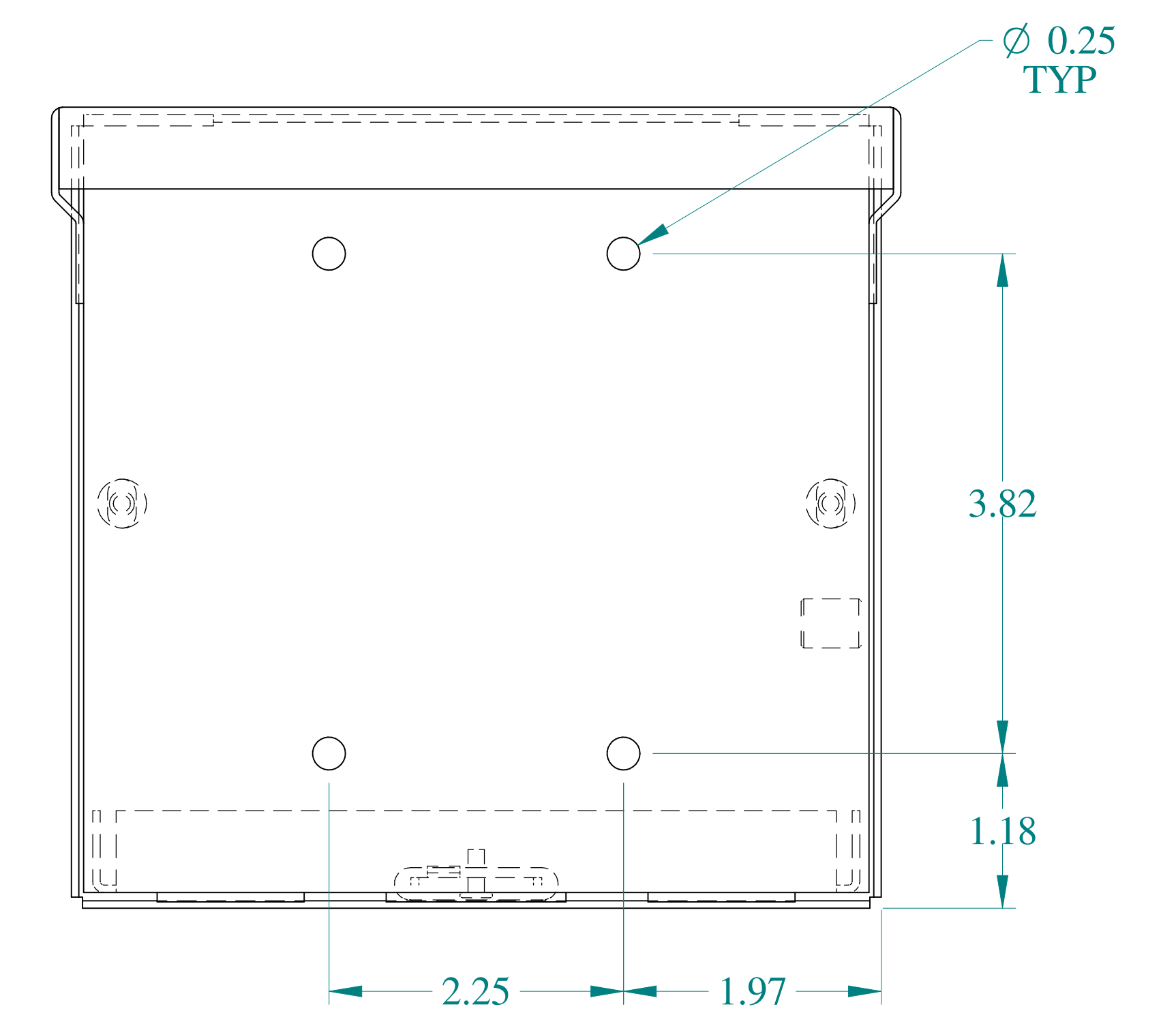
BACK VIEW
