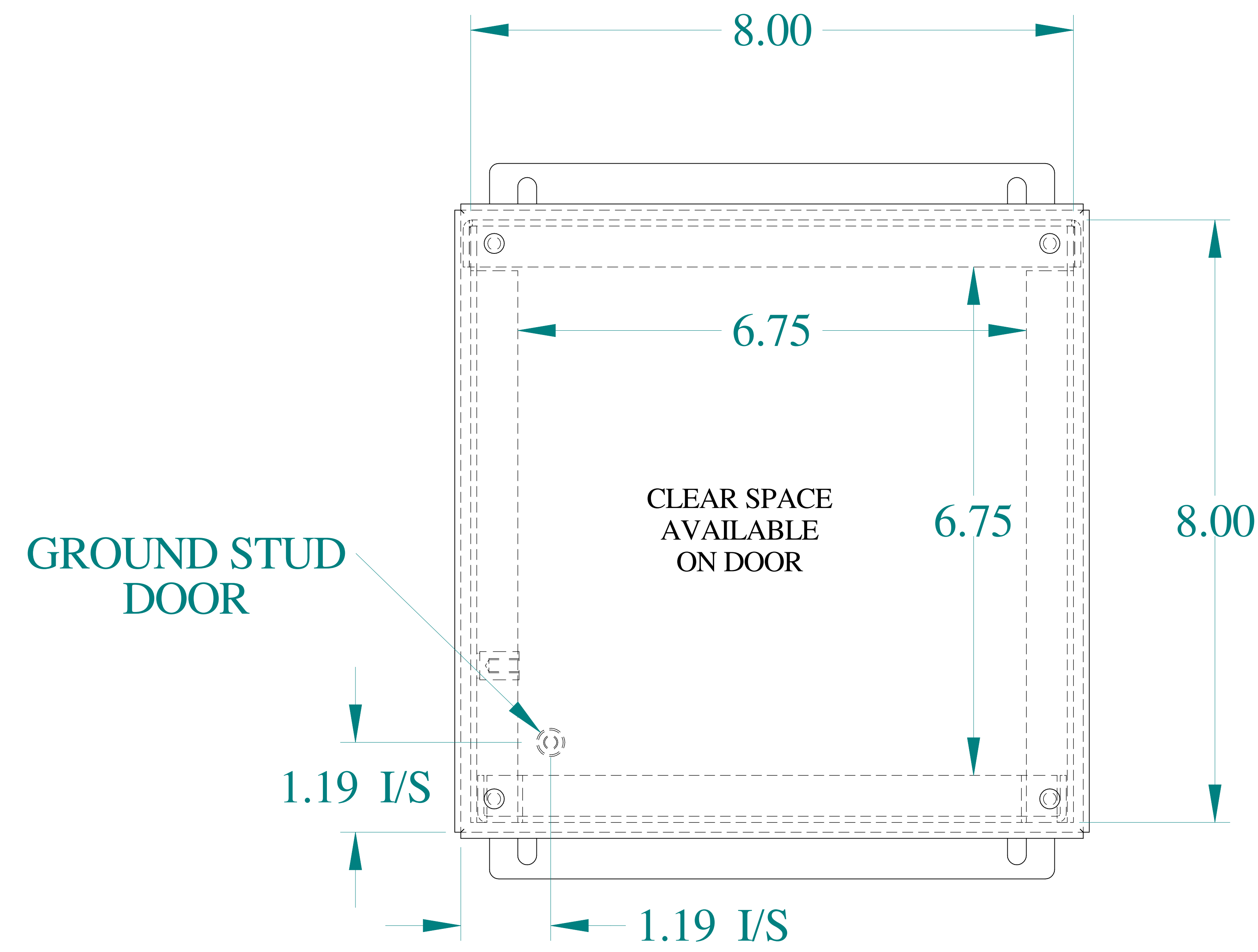
FRONT VIEW
