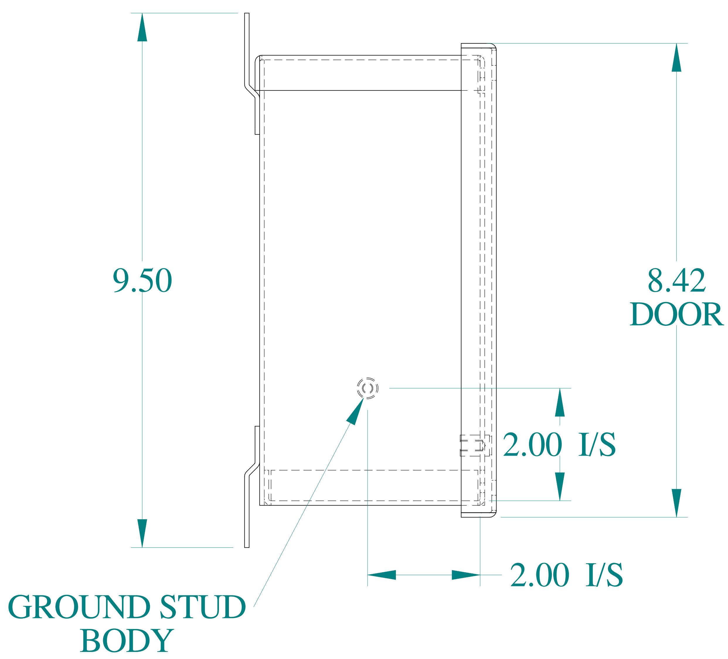
SIDE VIEW
