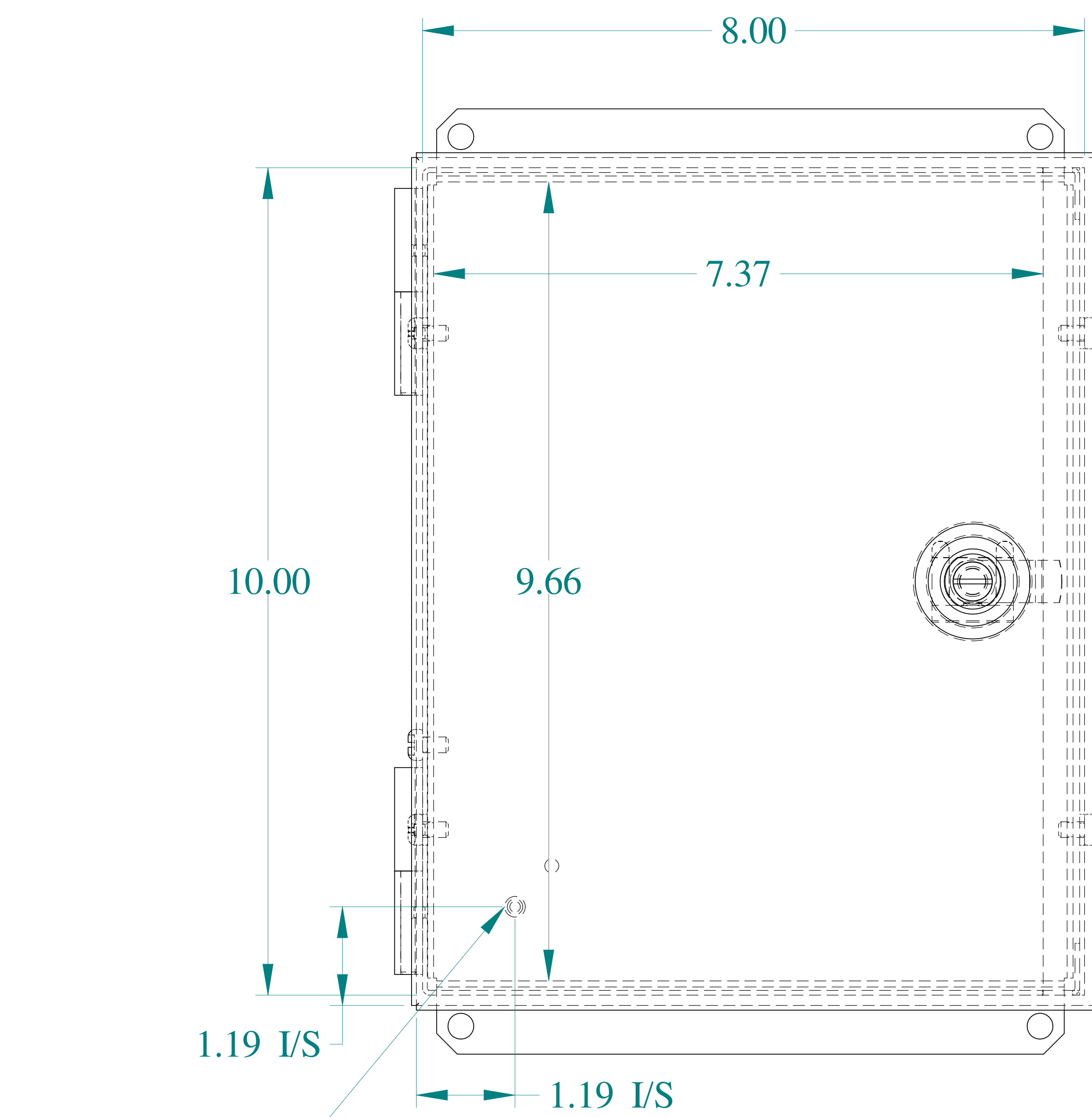
FRONT VIEW
