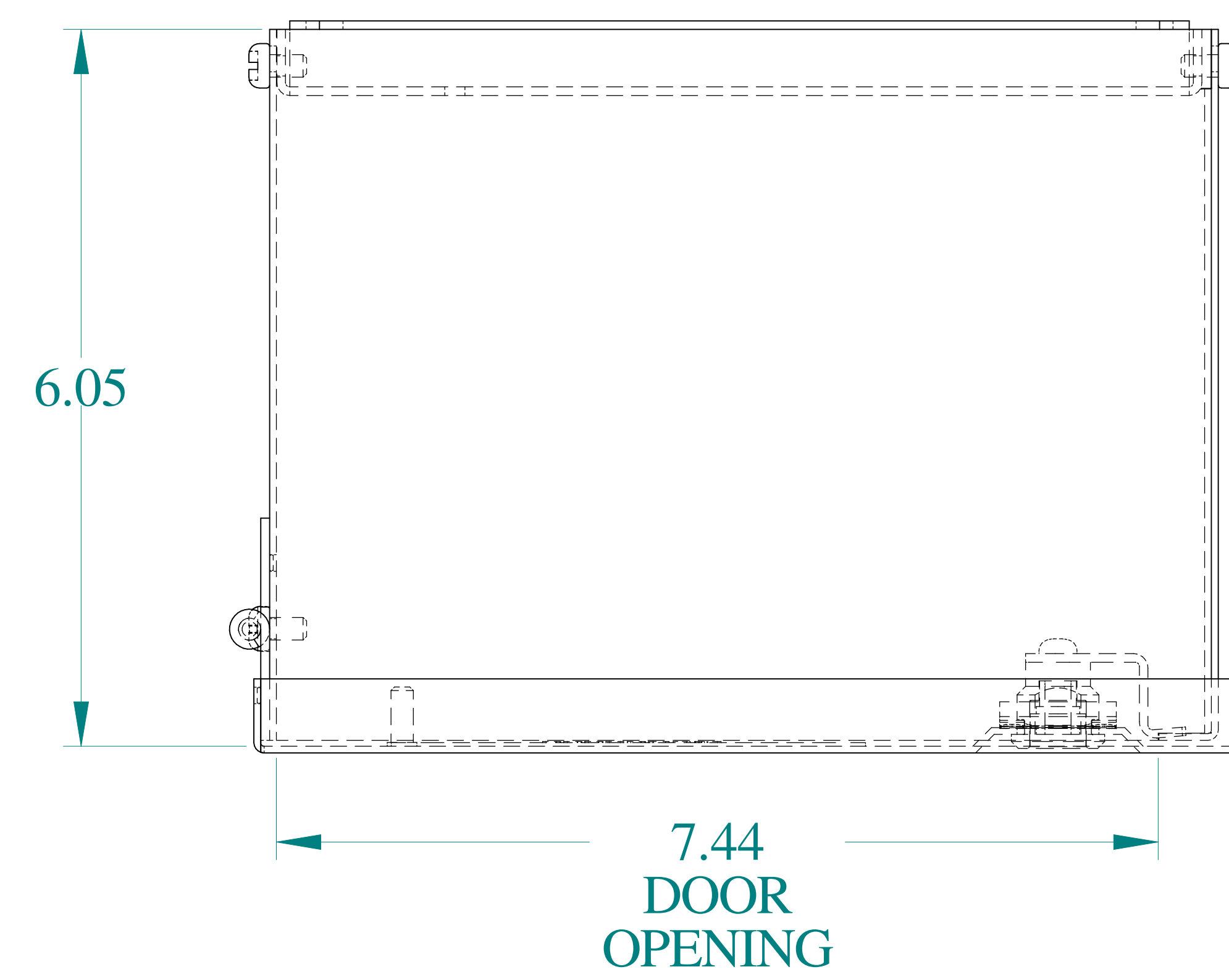
TOP VIEW
