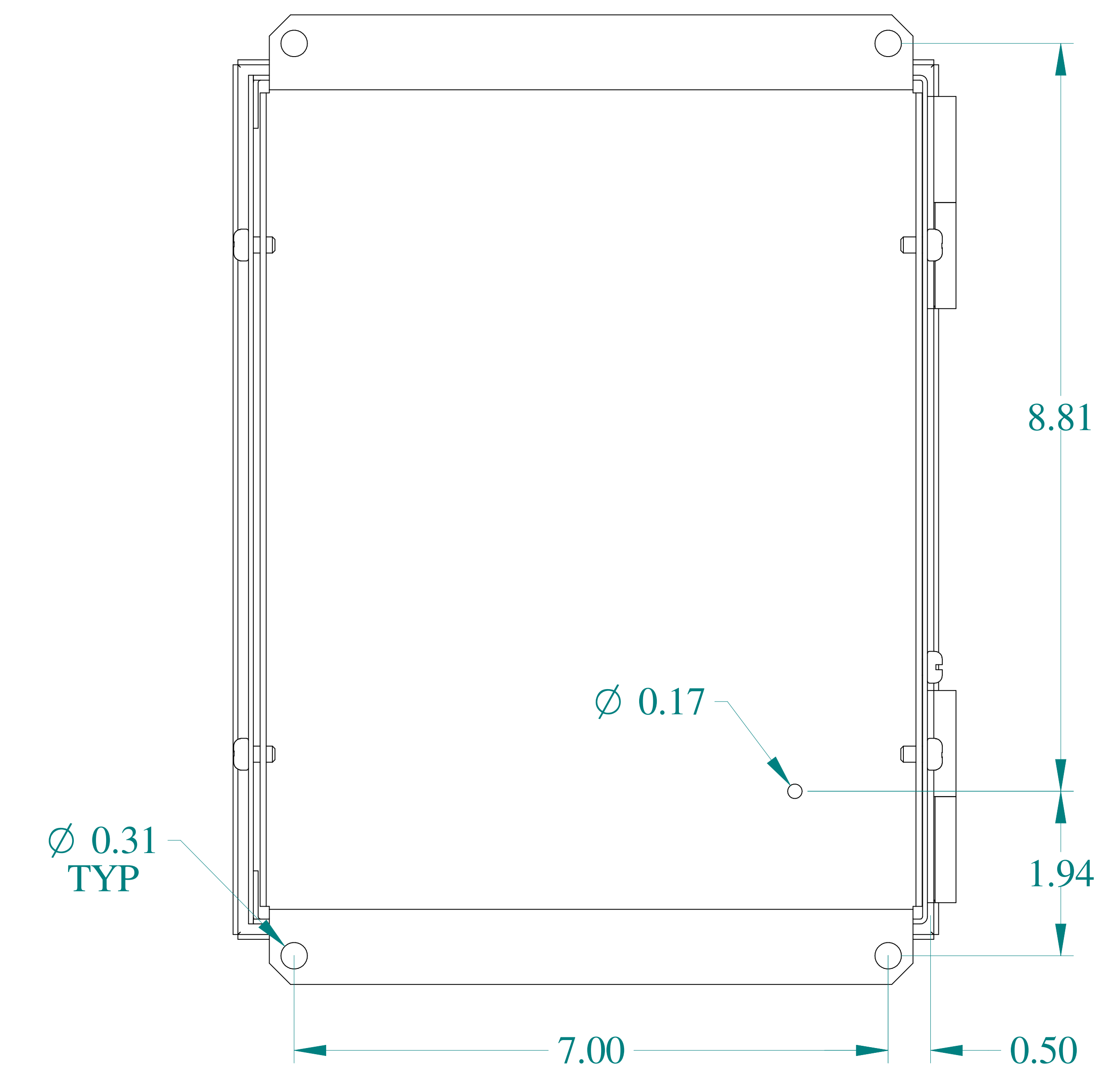
BACK VIEW
