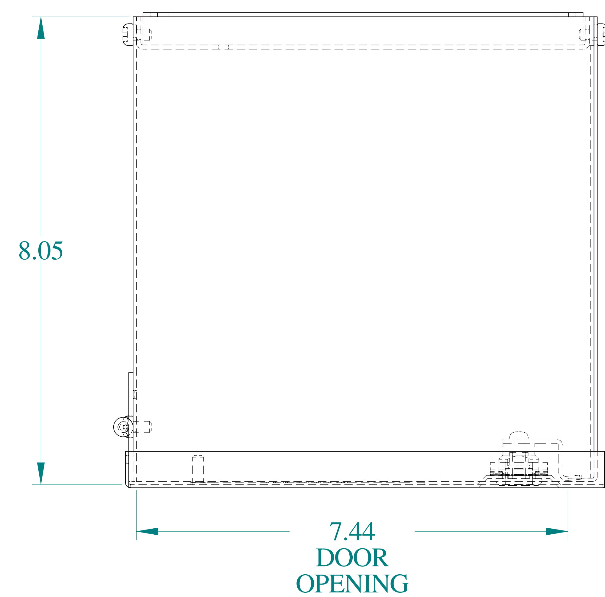
TOP VIEW
