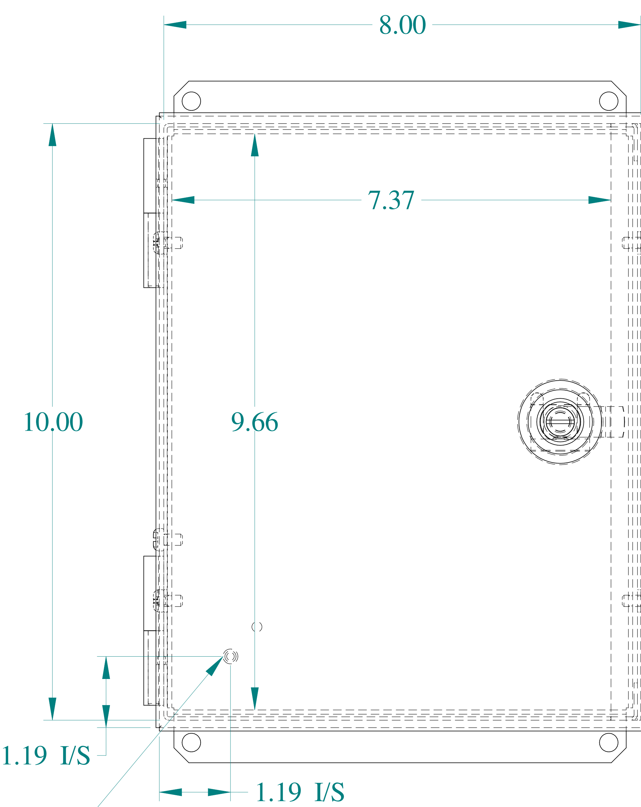
FRONT VIEW
