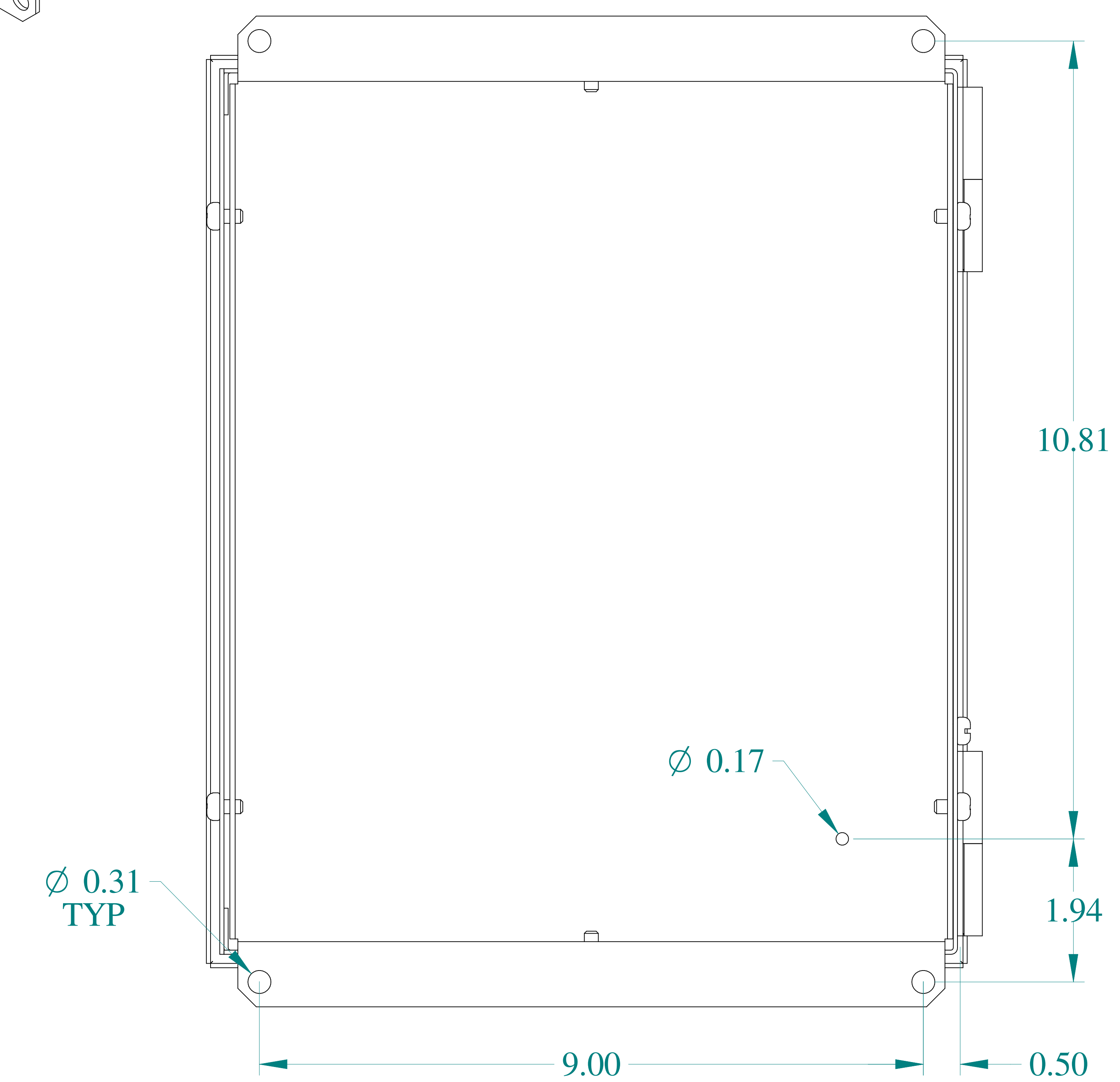
BACK VIEW
