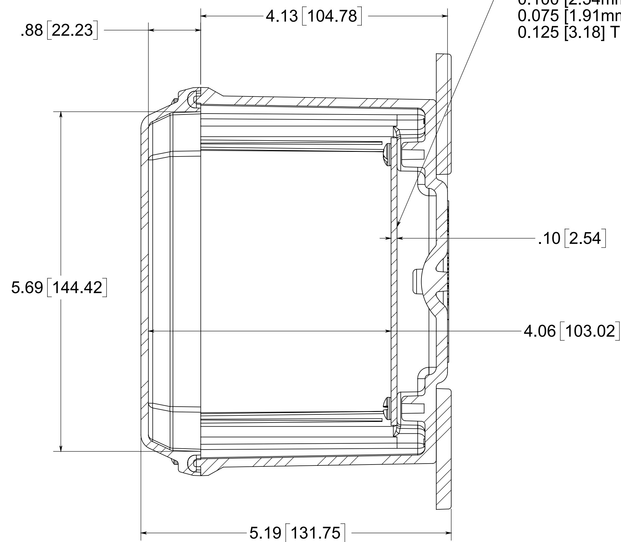
SECTION B-B
