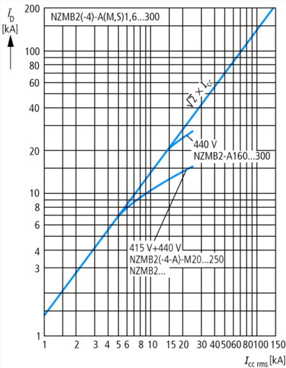
Let-through current
