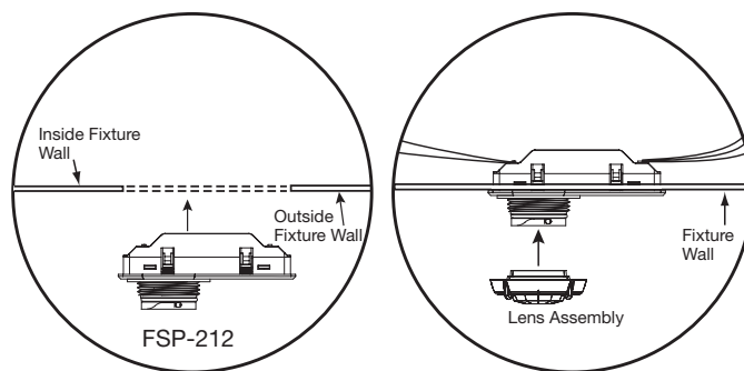
Snap-In Mounting
