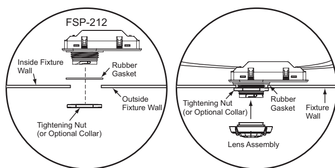
Threaded Collar Mounting
